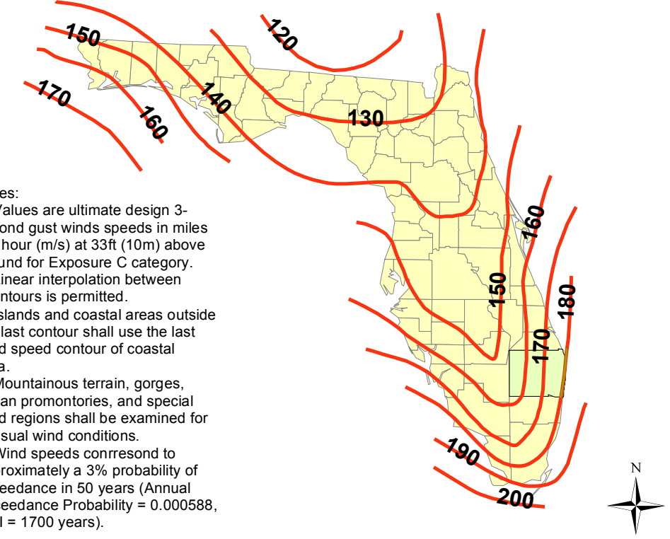
Figure 1609.3(2) Ultimate Design Wind Speeds, for Risk Category III and IV Buildings and Other Structures
