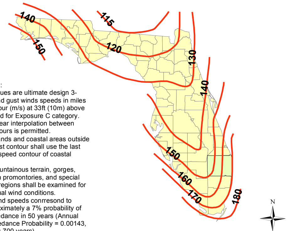
Figure 1609.3(1) Ultimate Design Wind Speeds, for Risk Category II Buildings and Other Structures
