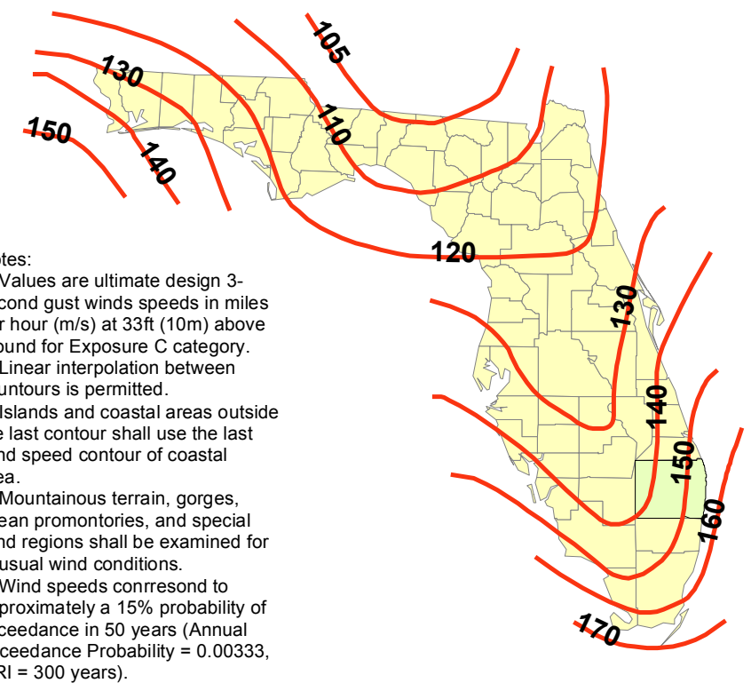
Figure 1609.3(3) Ultimate Design Wind Speeds, for Risk Category I Buildings and Other Structures
